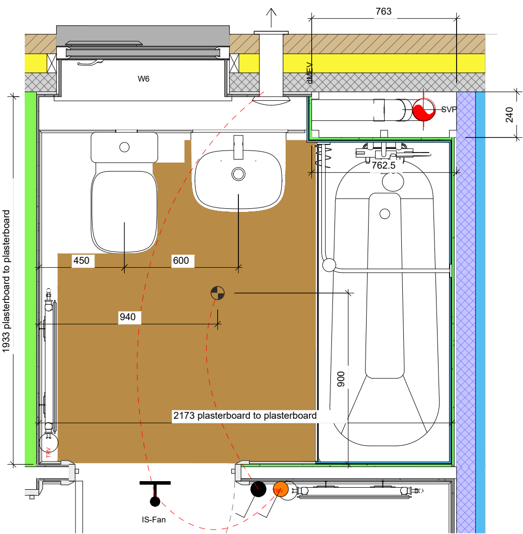
1 Bathroom Layout 1 : 20
